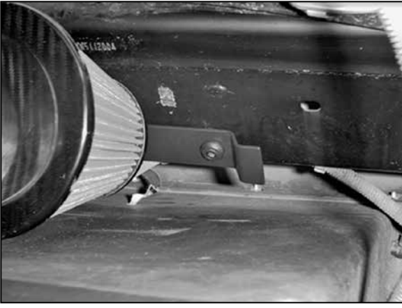
24. Install the angled bracket onto the original airbox mounting points.
